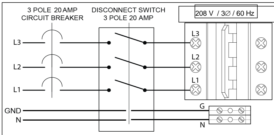
Figure 4-2 – CEN1600/2000: 208 V / 3Ø / 60 Hz - 5 Wire
