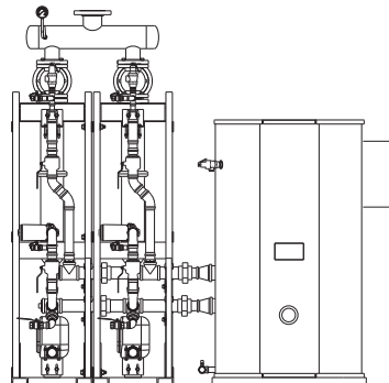
Dual Exchanger Configuration (Steam header and steam isolation valves are field-installed options)
